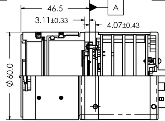
COMMON IMAGE PLANE DISTANCE
